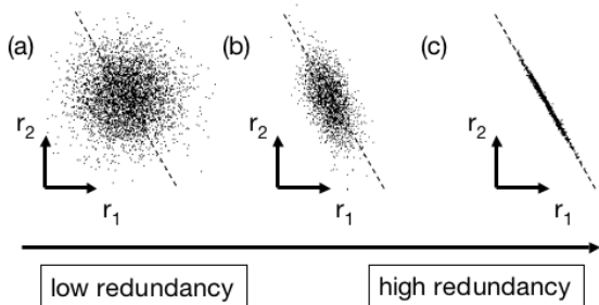
Figure 3: A spectrum of possible redundancies in data from the two separate recordings r_1 and r_2 (e.g. x_A, y_B ). The best-fit line r_2 = kr_1 is indicated by the dashed line.
